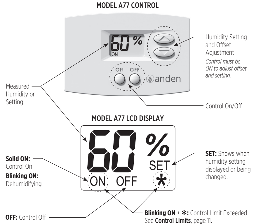
FIGURE 6 – EXTERNAL CONTROL
